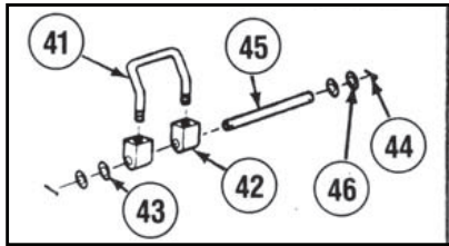
Safety Latch Assembly
